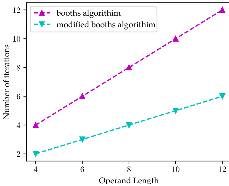
Figure 1: Iteration count of various operand lengths.
